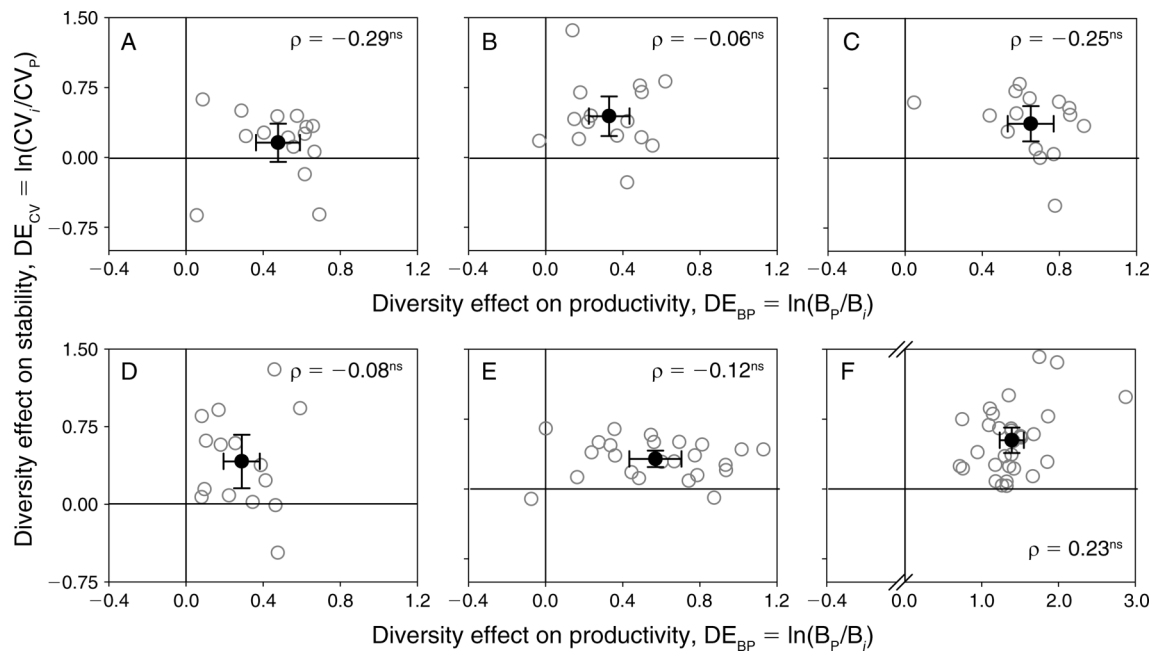
FIG. 3. Empirical relationship between the effect of producer diversity on production, and the effect of diversity on stability for six representative experiments. The x-axis in each plot gives the log ratio of biomass in any single experimental unit (e.g., a field plot) containing the most diverse polyculture relative to the same species grown in monoculture. The y-axis gives the log ratio of the coefficients of variation in any single experimental unit (e.g., a field plot) containing the most diverse polyculture relative to the same species grown in monoculture. Solid black circles give the mean effect sizes \pm 95\% confidence interval for all experimental units, and Spearman rank correlations ( \rho ) illustrate the covariance between the magnitude of the two diversity effects (ns indicates not significant). All data used to generate this figure are given in the Supplement in the file Data for within study analyses and come from the following sources: (A) Reich et al. (2001), BioCon E141 (ambient nitrogen, ambient CO_2 ); (B) Reich et al. (2001), BioCon E141 (enriched nitrogen, ambient CO_2 ); (C) Reich et al. (2001), BioCon E141 (ambient nitrogen, enriched CO_2 ); (D) Reich et al. (2001), BioCon E141 (enriched nitrogen, enriched CO_2 ); (E) Isbell et al. (2009); and (F) Tilman et al. (2001), Biodiversity II E120 experiment.
