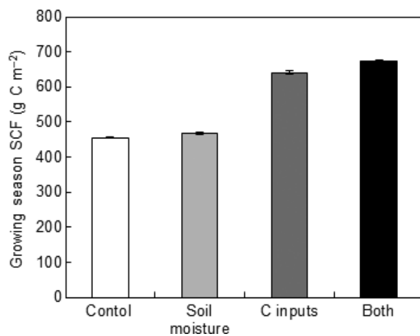
Fig. 9 Cumulative growing season soil C flux (growing season SCF) resulting from ambient CO 2 conditions (control, ambient CO 2 ), elevated CO 2 (eCO 2 ) soil moisture conditions (eCO 2 via soil moisture), eCO 2 C inputs (eCO 2 via C inputs), and eCO 2 soil moisture and C inputs (eCO 2 via C inputs + soil moisture). Cumulative growing season SCF was estimated using the predictions from the best model for describing SCF as a function of soil total soil water storage (TWS, 0–100 cm; Table 5; see Materials and methods). Error bars are \pm 1 SE.
