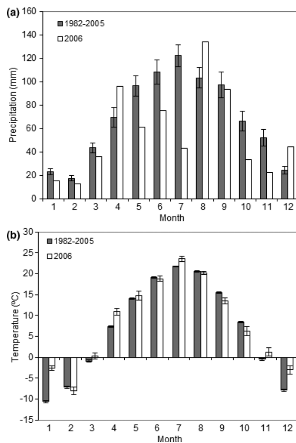
Fig. 2 Average monthly (a) precipitation and (b) temperature for 1982–2005 compared with (a) monthly precipitation and (b) mean monthly temperature in 2006. Error bars are \pm 1 SE.
