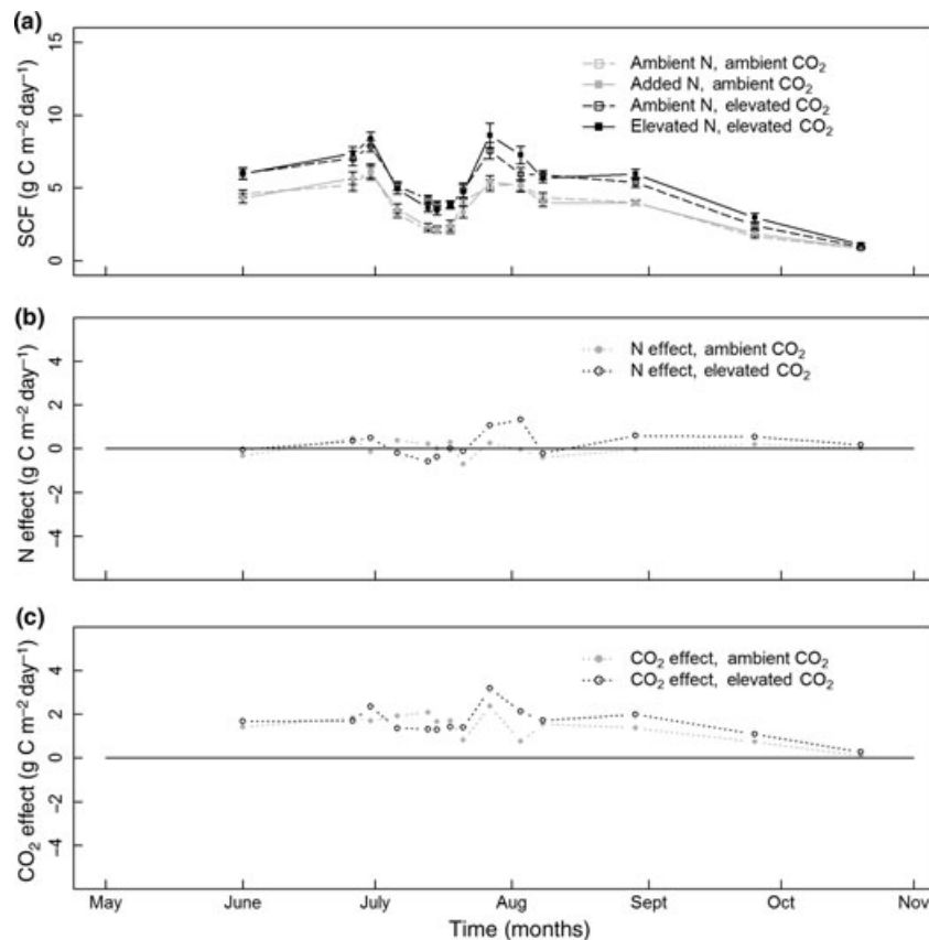
Fig. 7 Average soil carbon flux (SCF) by (a) CO 2 and N treatment and absolute (b) N and (c) CO 2 effects on SCF by N treatment. Absolute CO 2 and N effects were calculated as the mean SCF value for elevated CO 2 or N plots (by N or CO 2 treatment) minus the mean SCF value for ambient CO 2 or N treatments (by N or CO 2 treatment). In panels b and c, the solid black line without symbols indicates where the CO 2 or N effect is zero. Error bars are \pm 1 SE.
